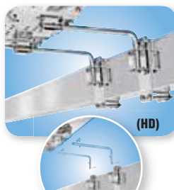
Extended "Dual" Side, Bulkhead or Square/Flat Rail Mount T10-640 Fits up to 2-1/4" (57 mm) sq. rail See website for application details Fits all ChefsMate, Newport, Catalina, & Monterey grills & "DM" tables
