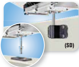
Socket Type Fish-Rod Holder Mounts T10-360 Fits Tempress Fish-On® & Roberts Rod Holder Sockets Fits 12" x 18" or smaller rect. grills & "SM" Tables Rod holder sockets not included.
