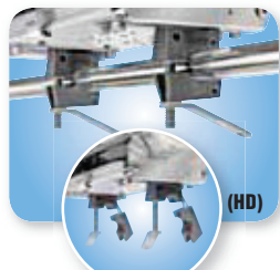
"Dual" Horizontal Round Rail Mount T10-580 Standard Rails 7/8" or 1" (22 mm or 25.5 mm) T10-585 Oversize Rails 1-1/8" or 1-1/4" (28.5 mm or 32 mm) T10-590 Large Rails 1-1/2" (38 mm) Fits all ChefsMate, Newport, Catalina & Monterey Grills & "DM" Tables
