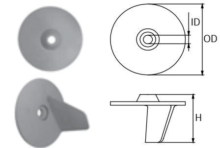
SUZUKI 115 HP
