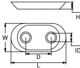
PLATE 2-8 HP
