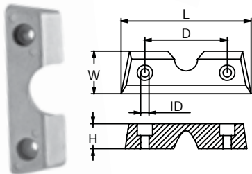
DPX SERIES
