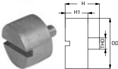
SEAL DRIVE 100
