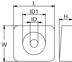
HONDA 8 - 10 - 15 HP
