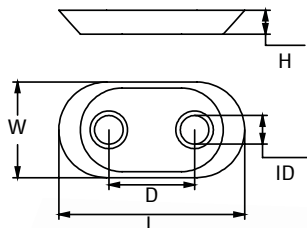
2-8 HP
