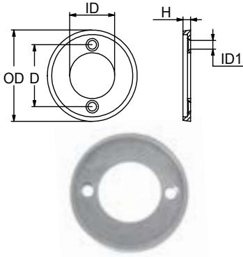
50-250-270-275-280-285 SERIES
