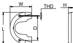
OMC 90 HP
