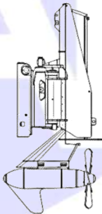
Type 2700 290 kW 2100 rpm
